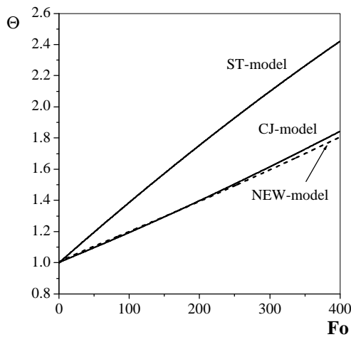
Figure 5: Time history of the mean temperature of an aluminum particle at T_{g\infty} = 1600 K
