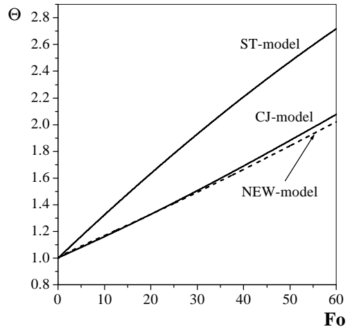
Figure 6: Time history of the mean temperature of a boron particle at T_{g\infty} = 1600 K
